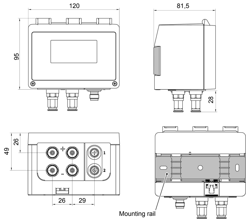
Fig. 5: Dimensional picture
