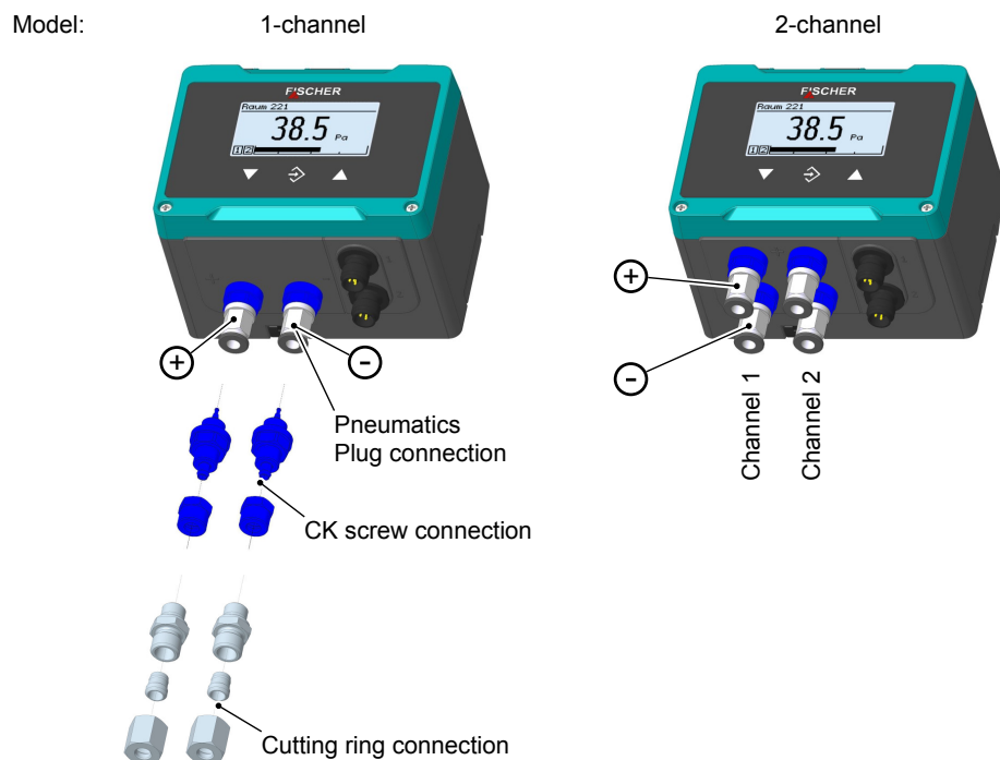
Fig. 2: Process connections
