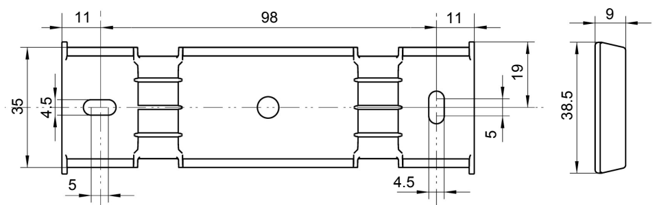
Fig. 6: Mounting rail
